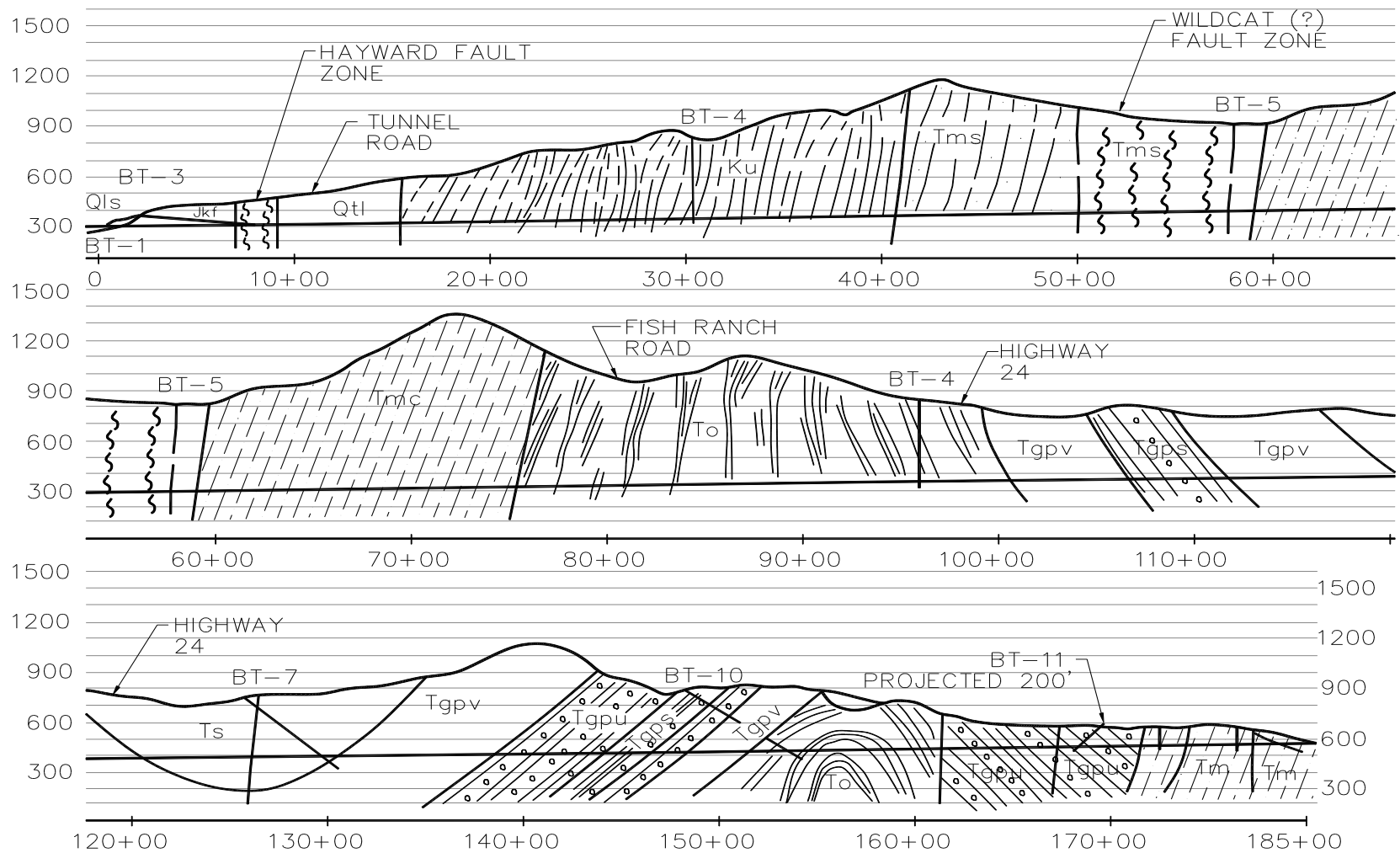
Figure 11.--Geologic profile along the 3.1-mile long Berkeley Hills Tunnel, which intercepts the Hayward fault about 700 feet in from the west portal. The tunnel was not designed for tectonic offset, but tracks have been continuously adjusted through the fault zone.
